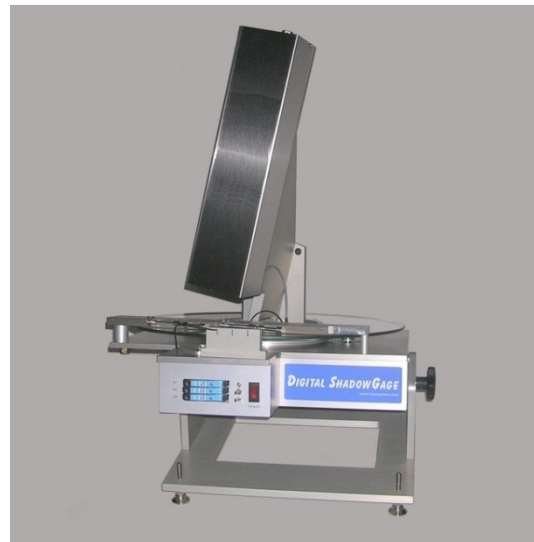
Model J197 with Camera Tilt Option
